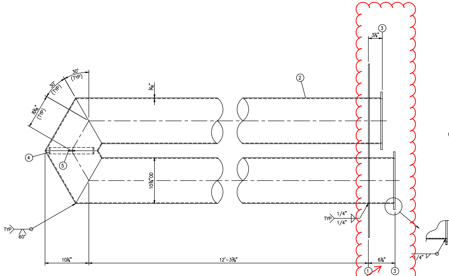
TOP VIEW
