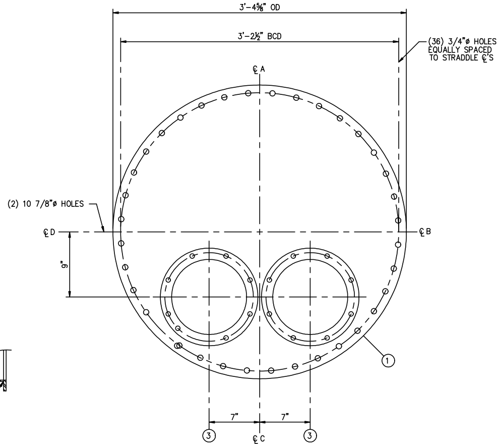
END VIEW
